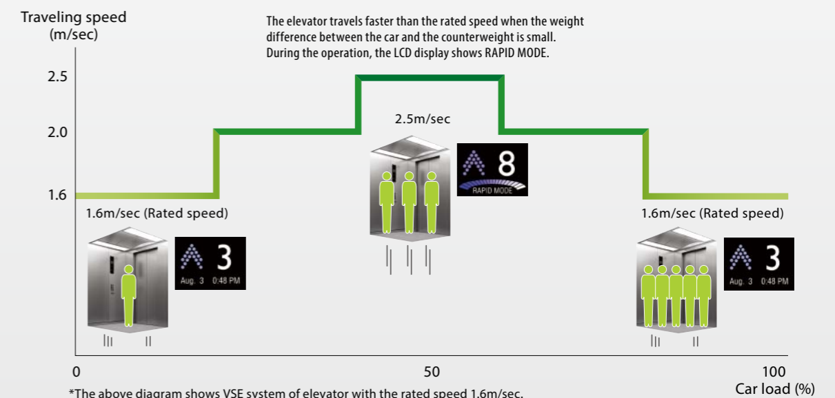
*The above diagram shows VSE system of elevator with the rated speed 1.6m/sec.
